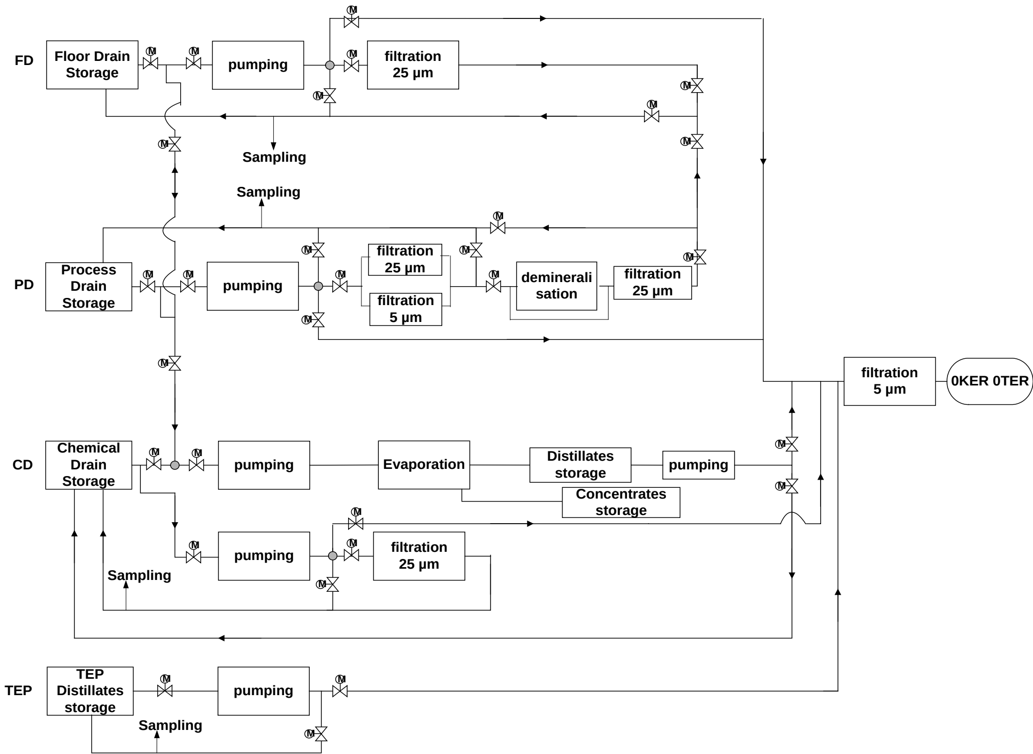
SECTION 6.4.2.2 - FIGURE 2: RULES FOR CHANNELLING EFFLUENT IN THE 8TEU [LWPS]
