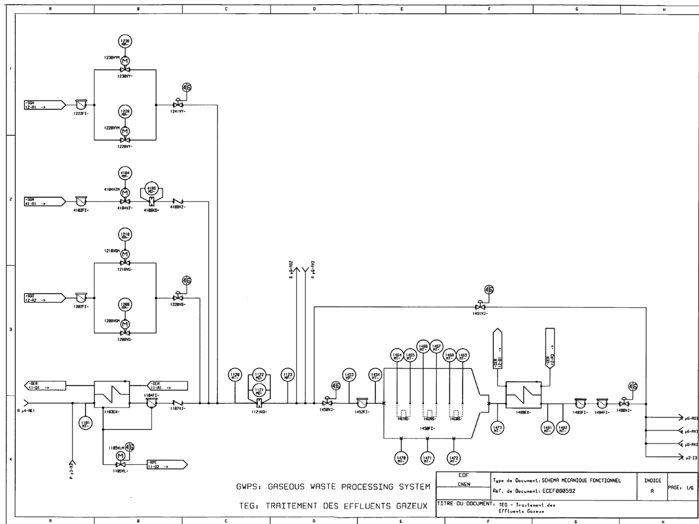
SECTION 6.4.3 - FIGURE 2 PAGE 1/6: TEG [GWPS] FUNCTIONAL FLOW DIAGRAM
