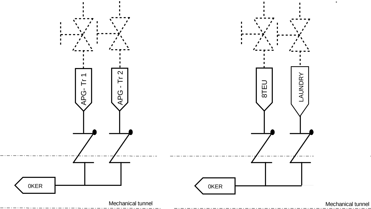
SECTION 6.4.2.3 - FIGURE 2: MECHANICAL DIAGRAM OF 0KER [LRMDS] COLLECTORS
