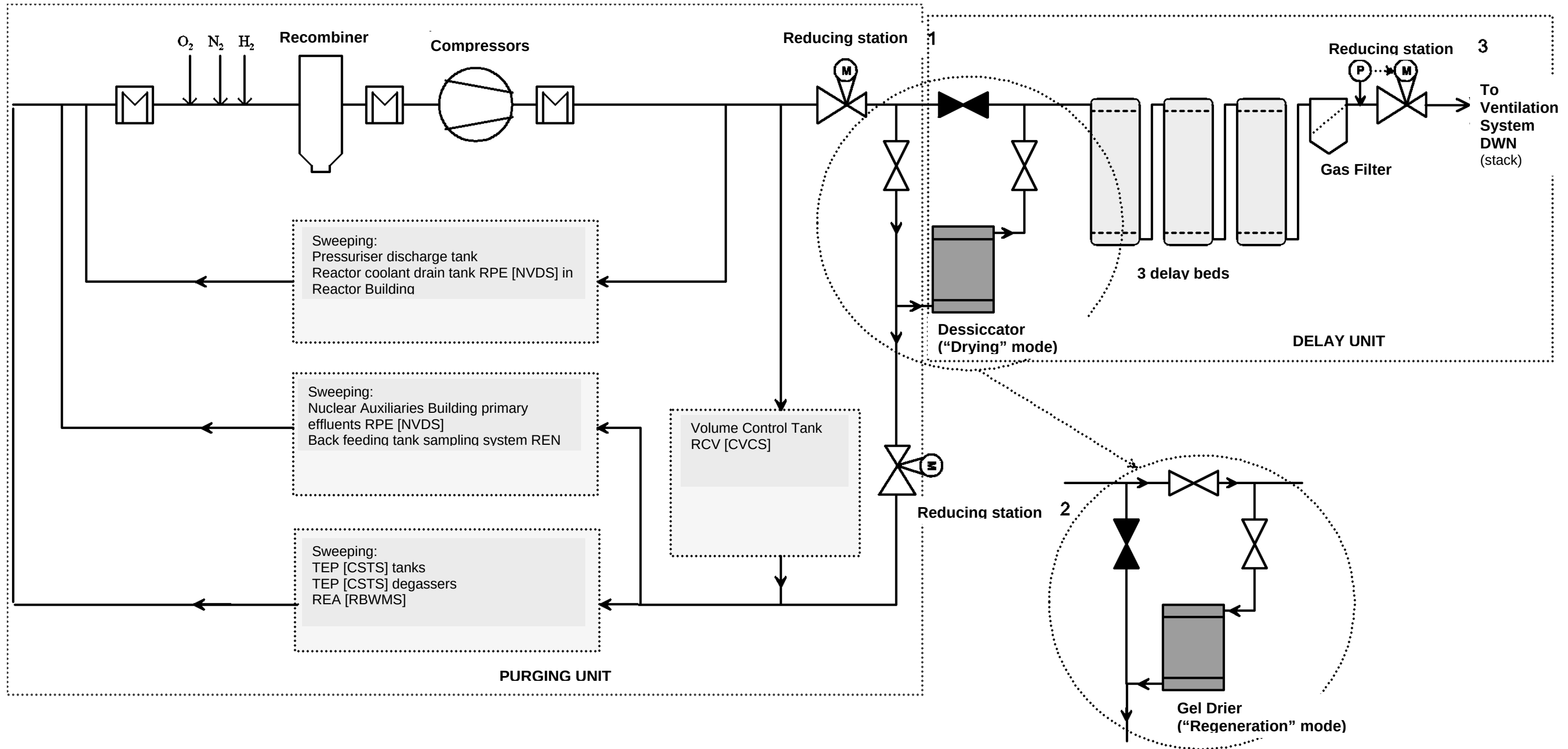
SECTION 6.4.3 - FIGURE 1: SIMPLIFIED DIAGRAM OF THE TEG [GWPS] SYSTEM
